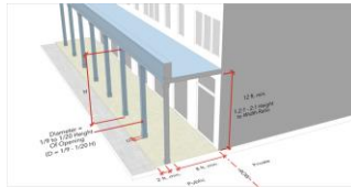
ILLUSTRATION 12-3-31.8. GALLERY ENCROACHMENTS
