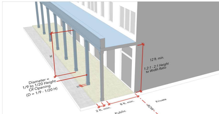
Illustration 12-2-25.8 - Gallery Encroachments
