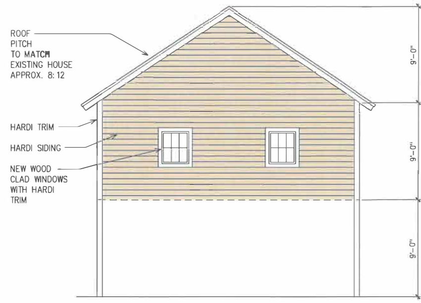
2 WEST ELEVATION A2 1/4"=1'-0"
