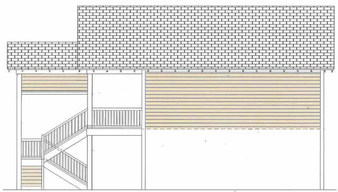
3 NORTH ELEVATION A2 1/4"=1'-0"
